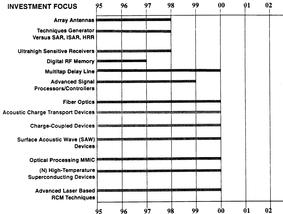
Figure 5-8. Key Technologies Roadmap Surface Tactical EW Systems
